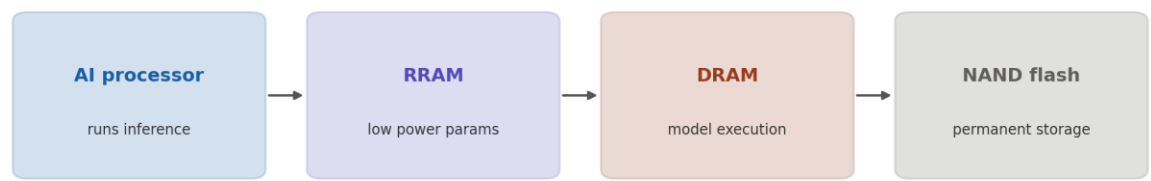
Models load from NAND into DRAM; frequently used parameters are kept in RRAM
